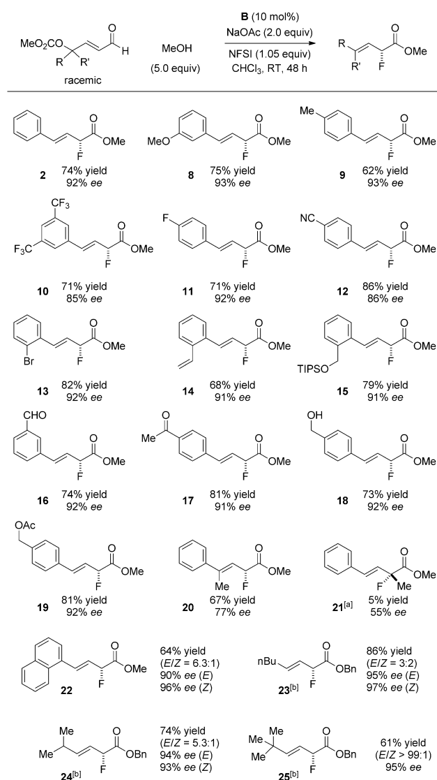
Scheme 2. Scope of the fluorination reaction in \alpha position. Yields of purified products are given. [a] The starting material (> 90%) was recovered. [b] 5.0 equiv of BnOH was used instead of MeOH, because of the low boiling point of the methyl ester product. Bn = benzyl, TIPS = triisopropylsilyl.
